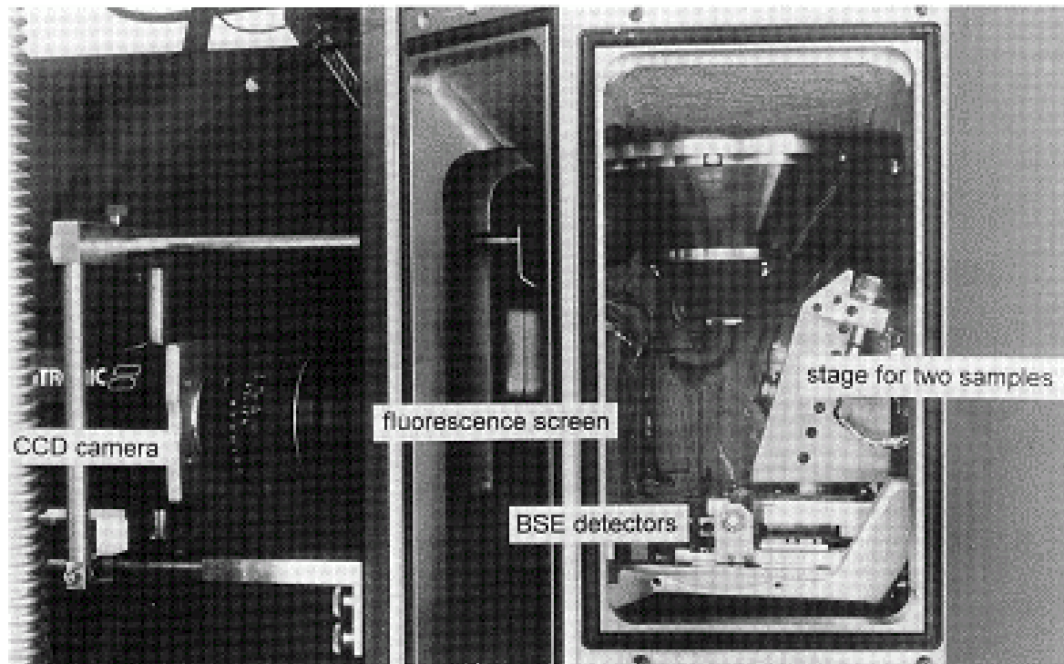
Fig. 2. Experimental set-up for the acquisition of backscatter Kikuchi patterns with a JBOL JSM 6400 SEM.
